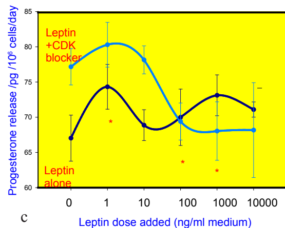
Fig. 2: Effect of leptin (0, 1, 10, 100, 1,000 or 10,000 ng/ml medium) with and without presence of cyclin-dependent protein kinase blocker, olomoucine, on the release of arginine-vasotocin (a), estradiol (b) and progesterone (c) by cultured chicken ovarian granulosa cells. Values were obtained by combination of RIA/EIA as indicated in Materials and Methods. Values are means + S.E.M. * P < 0.05 vs. control group (medium without leptin)
