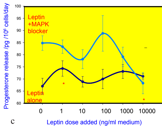
Fig. 1: Effect of leptin (0, 1, 10, 100, 1,000 or 10,000 ng/ml medium) with and without presence of mitogen activated protein kinase blocker, PD98059, on the release of arginine-vasotocin (a), estradiol (b) and progesterone (c) by cultured chicken ovarian granulosa cells. Values were obtained by combination of RIA/EIA as indicated in Materials and Methods. Values are means + S.E.M. * P < 0.05 vs. control group (medium without leptin)
